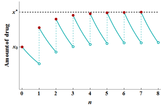
Figure 6: Amount of drug in the body where a dose of size b is administered every \tau time units. The red points show the values of x_n where n represents n\tau time units, the blue curves show the decay of the drug between doses, and x^* represents the equilibrium value.
