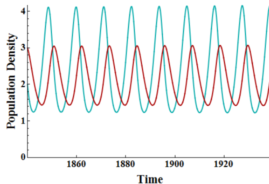
Figure 13: Plot of the sequences produced by the discrete Lotka-Volterra model, Equations (29) - (30), with r = 1.0015 , s = 0.9994 , \alpha = 0.0006 , \beta = 0.00025 , and each time step represents 14.6 hours (a little more than half a day).
