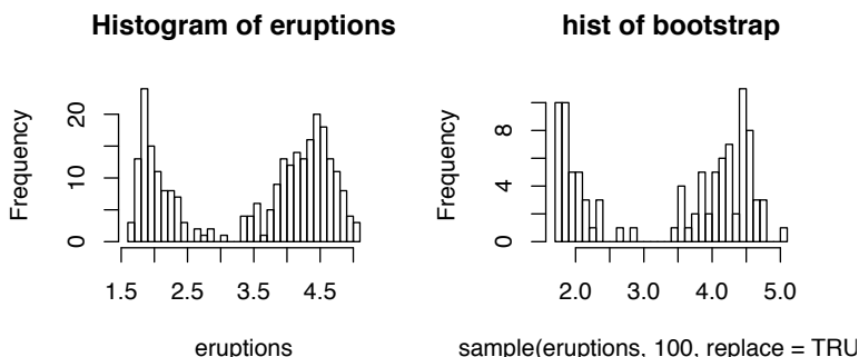
Figure 29: Bootstrap sample
