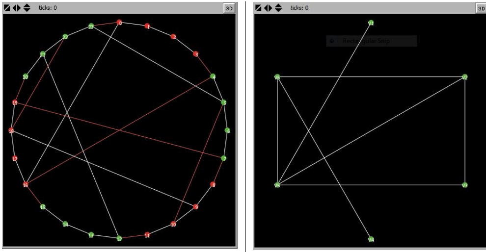
Figure 1: The left panel shows an instance of G_{SW}^1(24, 1, 0.5) . The right panel shows a corresponding graph G_I .
